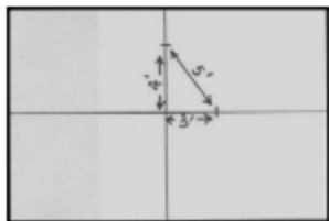
Figure 1 To square the area to be covered, first find the center of one end of the main rectangle. Locate the same point at the other end wall. Snap a chalk line between these points to mark the center line on the floor. Then measure along this center line to find the middle of the room. At the center point, mark off a line across the room at exactly right angles to the first line. This may be accomplished by the 3-4-5- triangle method as shown in Figure 1 . Then measure 4 feet toward each side wall from the center point. Then measure 3 feet from the center point along the longer line, measure exactly 5 feet from the 3 foot mark on the center line to the 4 foot mark on the cross line. If the 5 foot measurements do not come out exactly 5 feet, the center crossing lines are not at a true right angle. For large rooms, multiples of the above dimensions may be used to obtain greater accuracy. (6-8-10 or 9-12-15, etc.)
